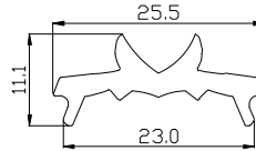
Model No.:ASEL26D180G Material:PMMA 50% Beam Angle:180°
