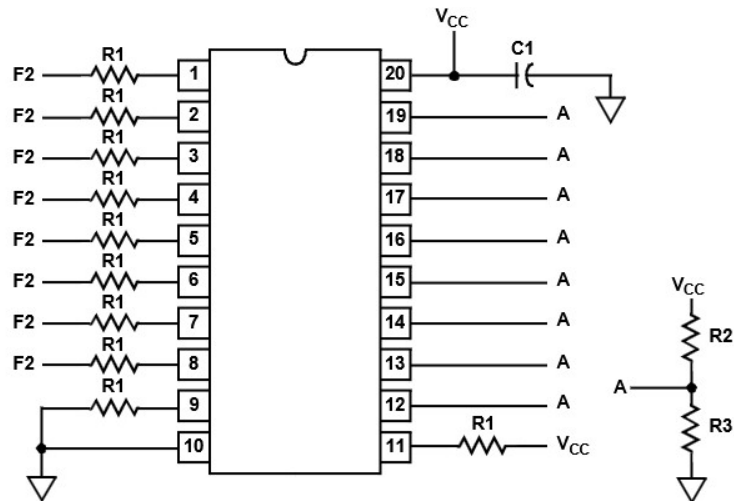
MD82C86H CERDIP
