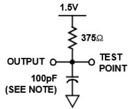
TELOV OUTPUT HIGH ENABLE LOAD CIRCUIT
