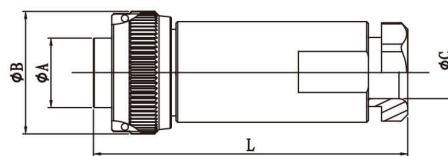
带尾附电缆插头 Cable plug with tail
